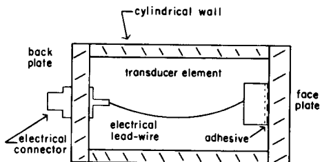
FIG. 2 Basic Features of a Housed Transmitter or Receiver
